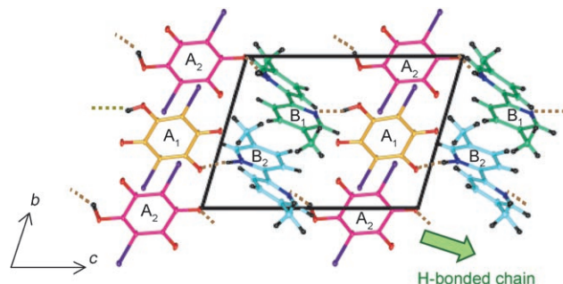
Figure 1. The crystal structure of [H-55DMBP][Hia] at 50 K viewed along the a axis. The acid ( A 1 and A 2 ) and base ( B 1 and B 2 ) molecules are connected into chains by hydrogen bonds (dashed lines). The direction of propagation of the chains is indicated by the green arrow. C yellow ( A 1 ), pink ( A 2 ), green ( B 1 ), or blue ( B 2 ); H black, N blue, O red.
