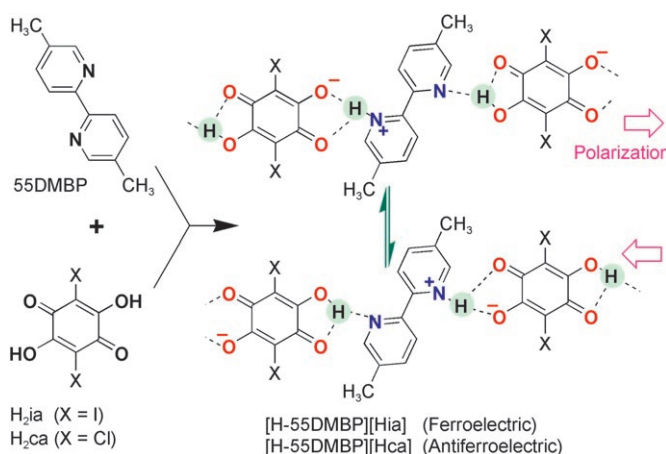
Scheme 1. The formation of polar chains of alternating acid and base molecules through hydrogen bonding (dashed lines) and the reversal of their polarization through a cooperative transfer of protons (green circles).
